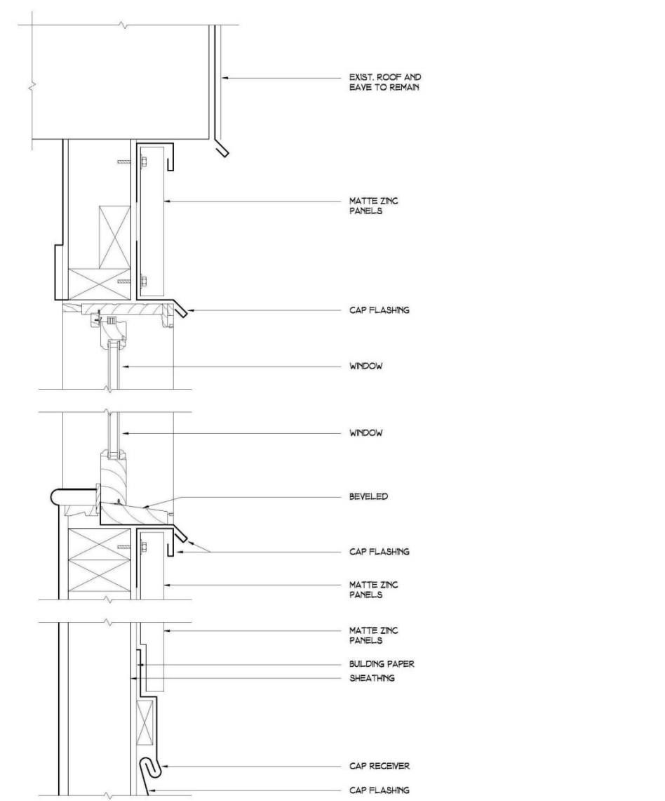
WINDOW DETAIL AT PENTHOUSE WALL
