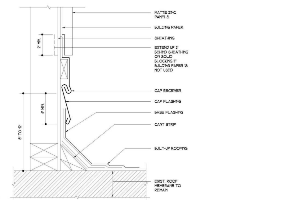
FLASING/WATER PROOFING DETAIL AT PENTHOUSE WALL
