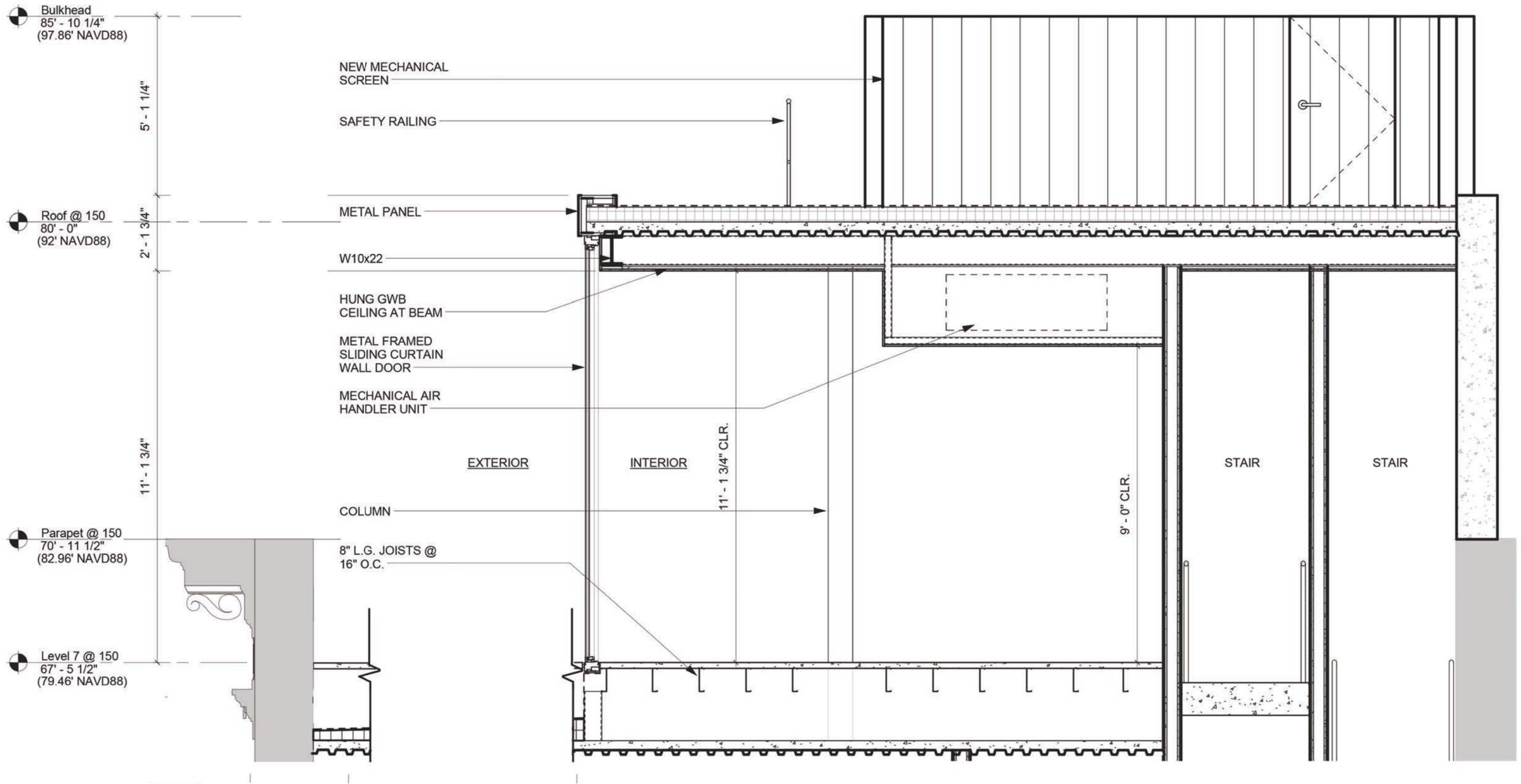
Proposed Roof Addition Section
