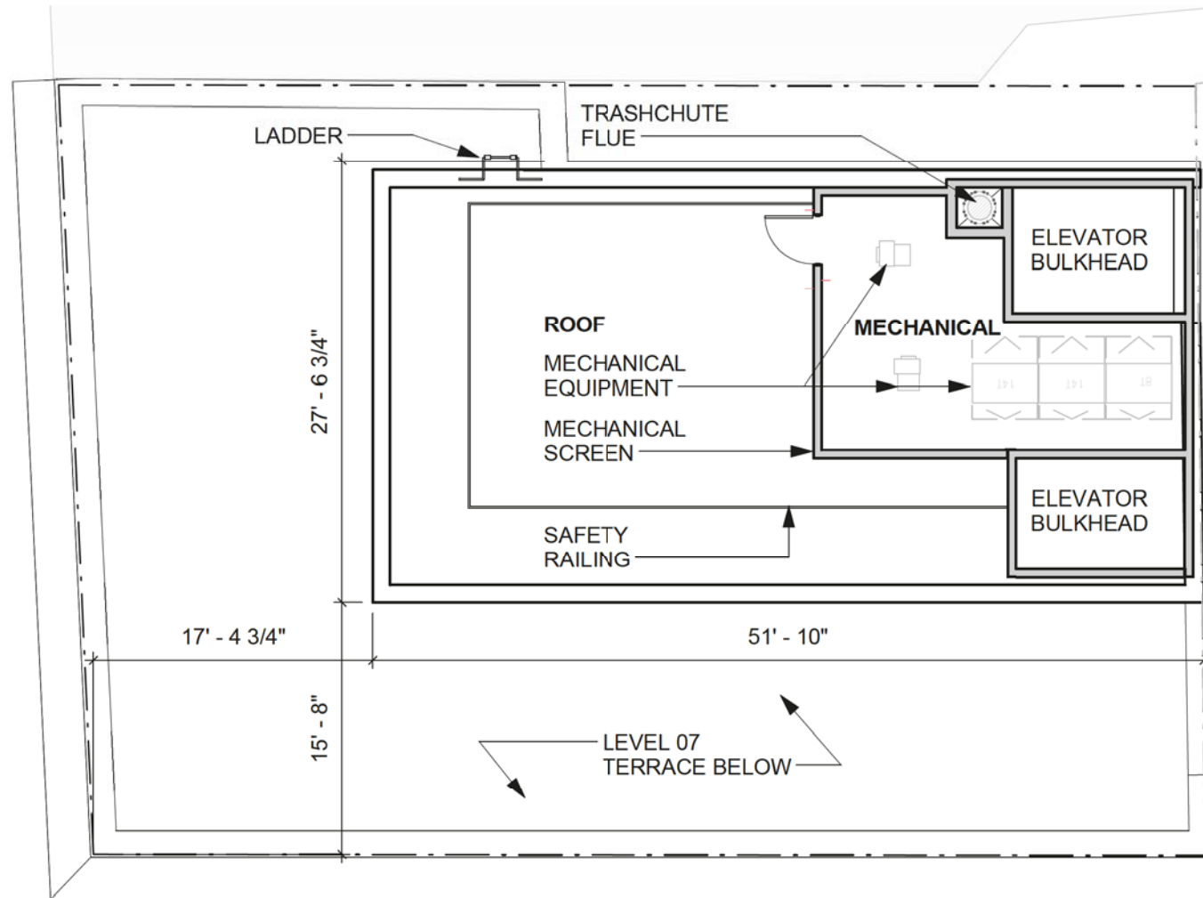
Originally Proposed Level 07 Plan
