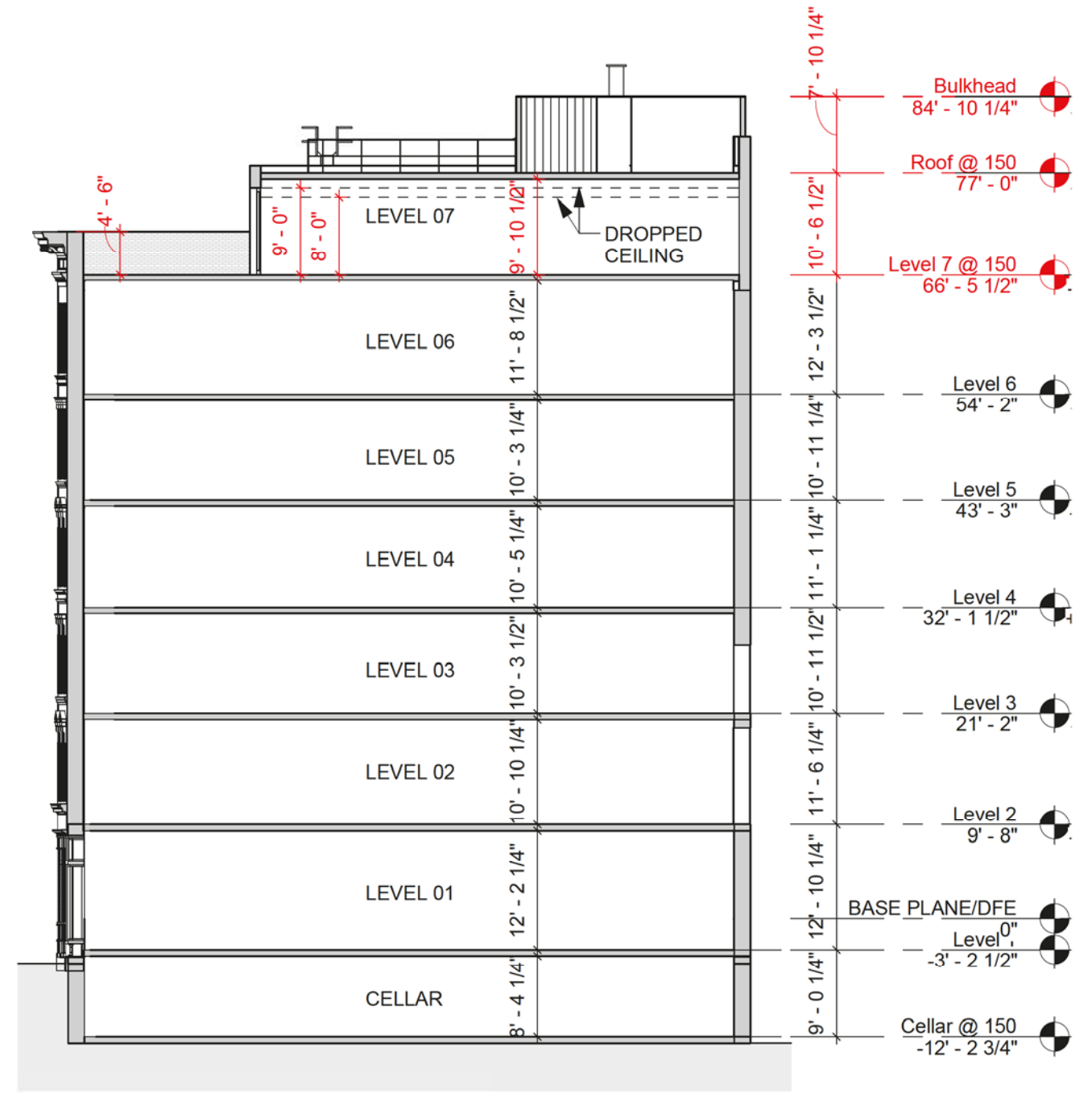
Revised Building Section
