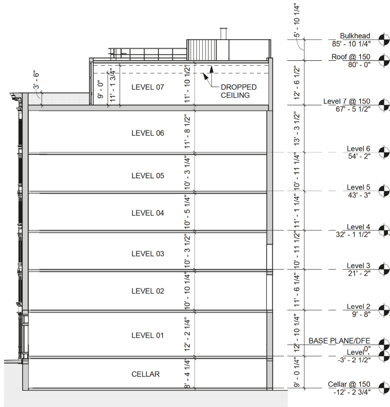
Originally Proposed Building Section
