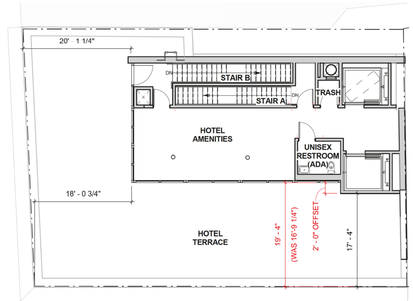
Revised Level 07 Plan
