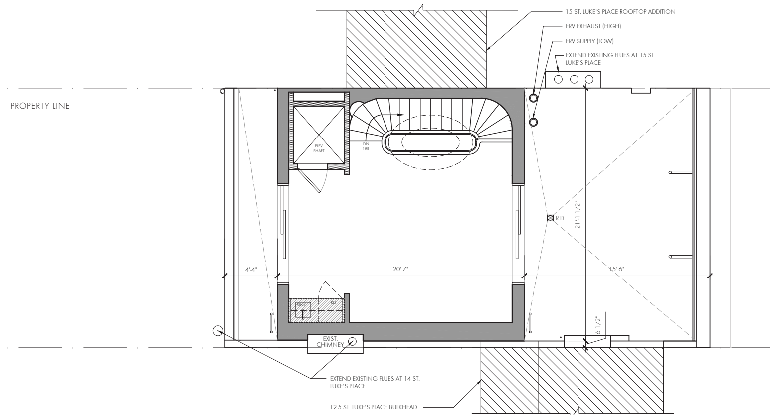
PROPOSED ROOFTOP ADDITION PLAN
