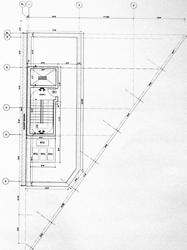
1 Roof Plan
