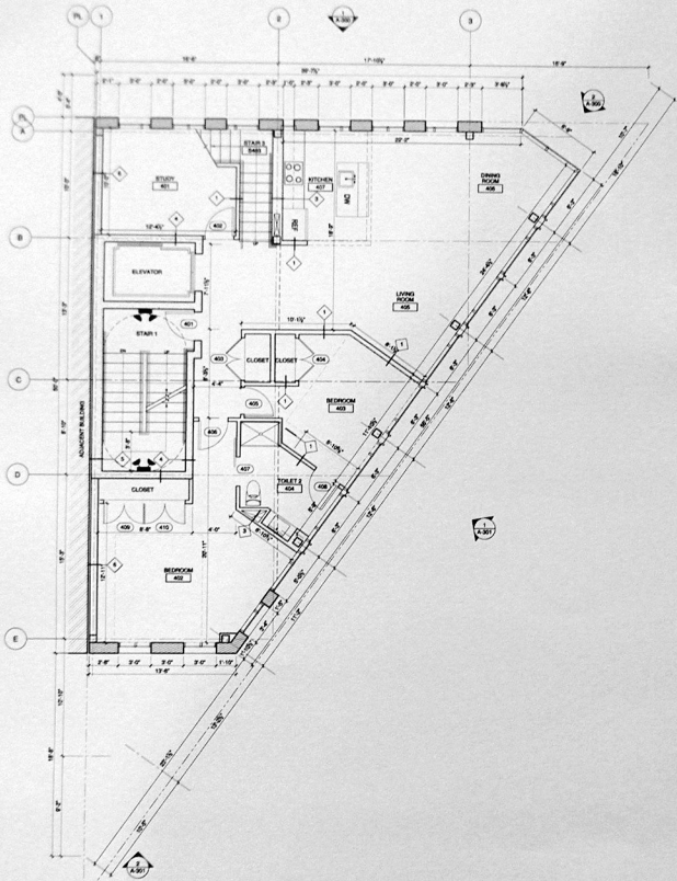
1 Fourth Floor Plan
