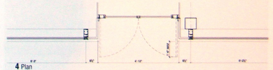
4 Plan
