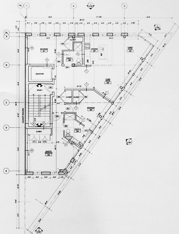
2 Third Floor Plan
