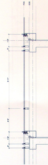
2 Section
