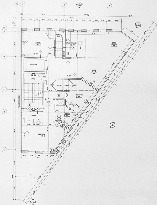
1 Fourth Floor Plan
