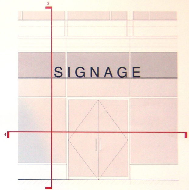
3 Detail Elevation At Entry
