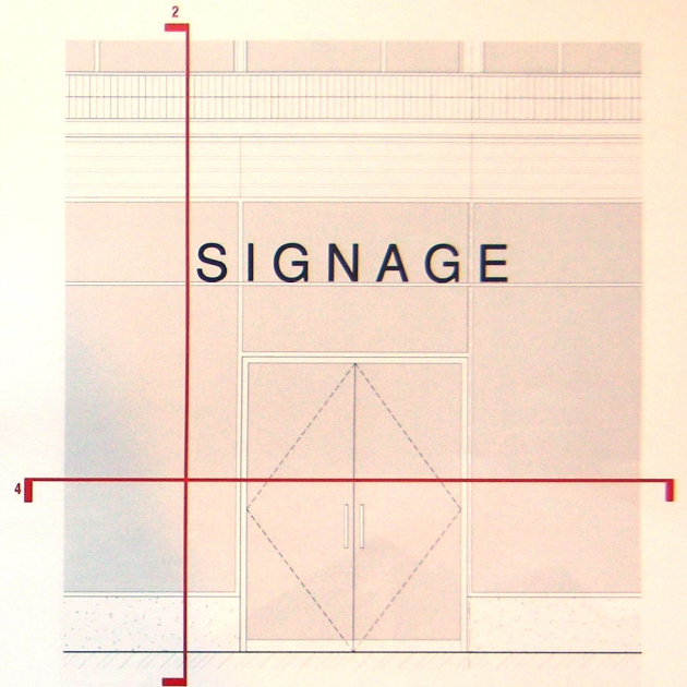
3 Detail Elevation At Entry
