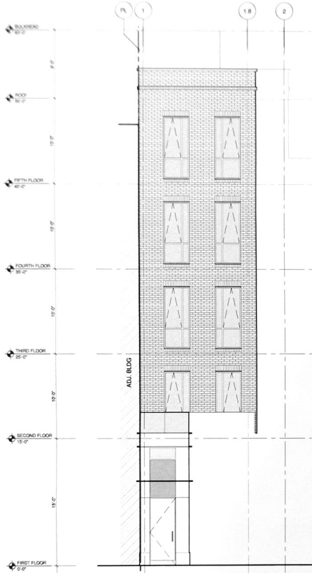
1 Rear Elevation
