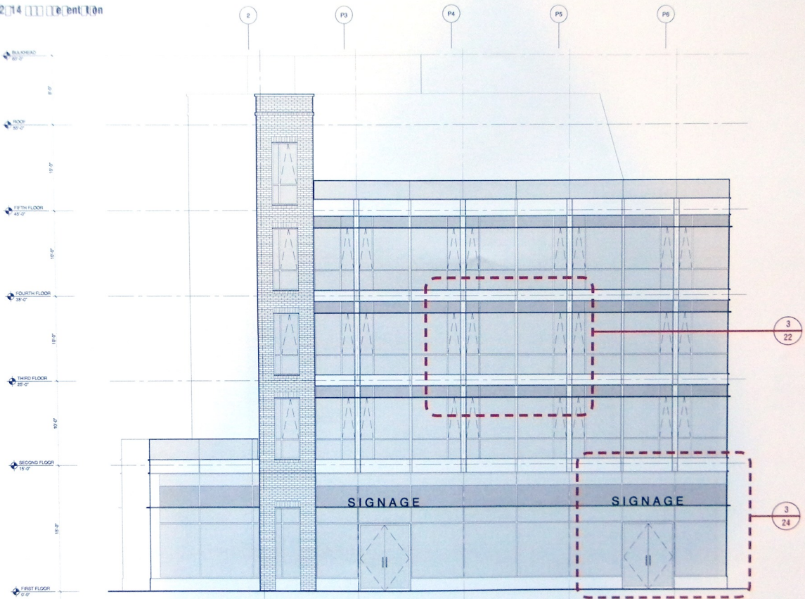
1 Seventh Avenue South Elevation
