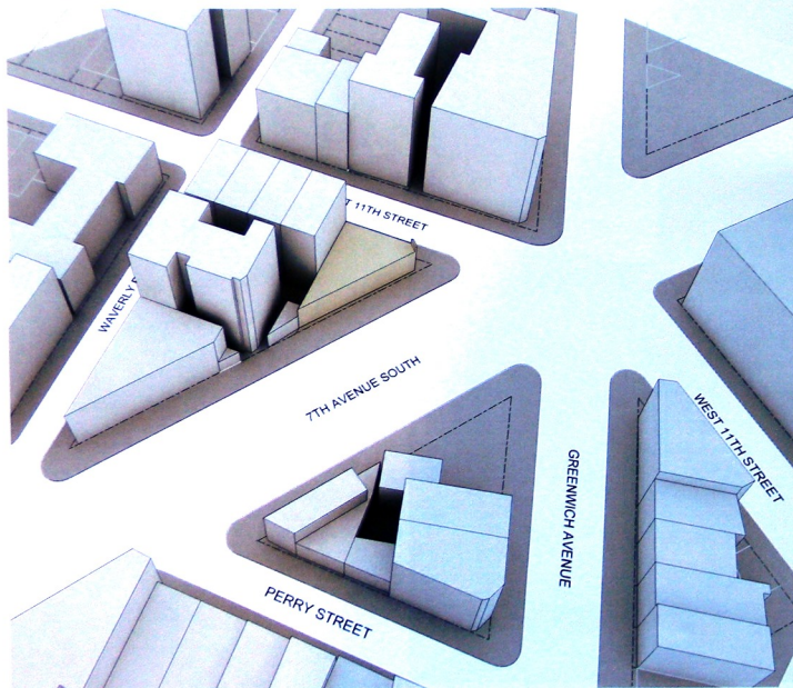
1 Existing Area Massing
