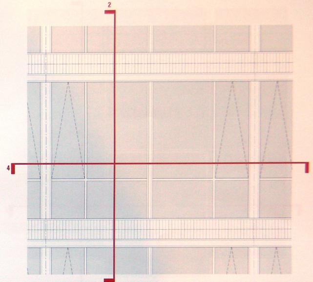
3 Typical Curtain Wall Elevation
