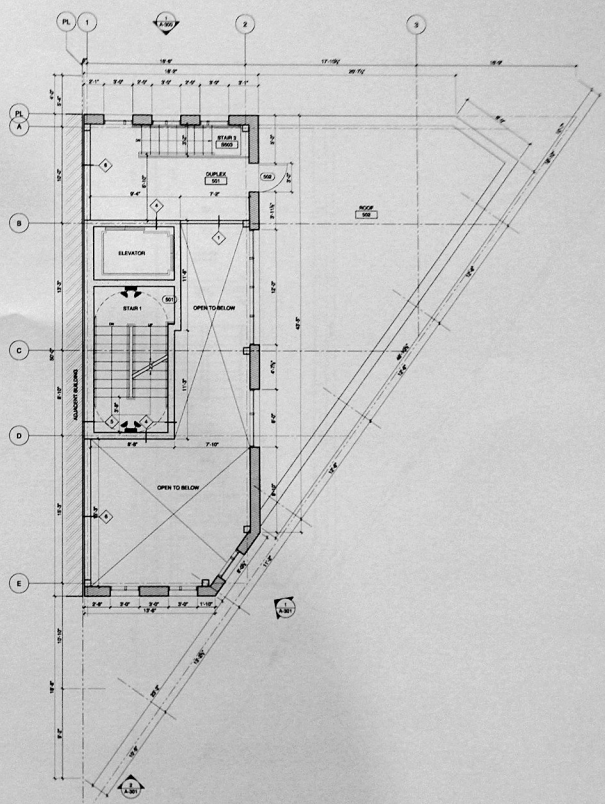
2 Fifth Floor Plan
