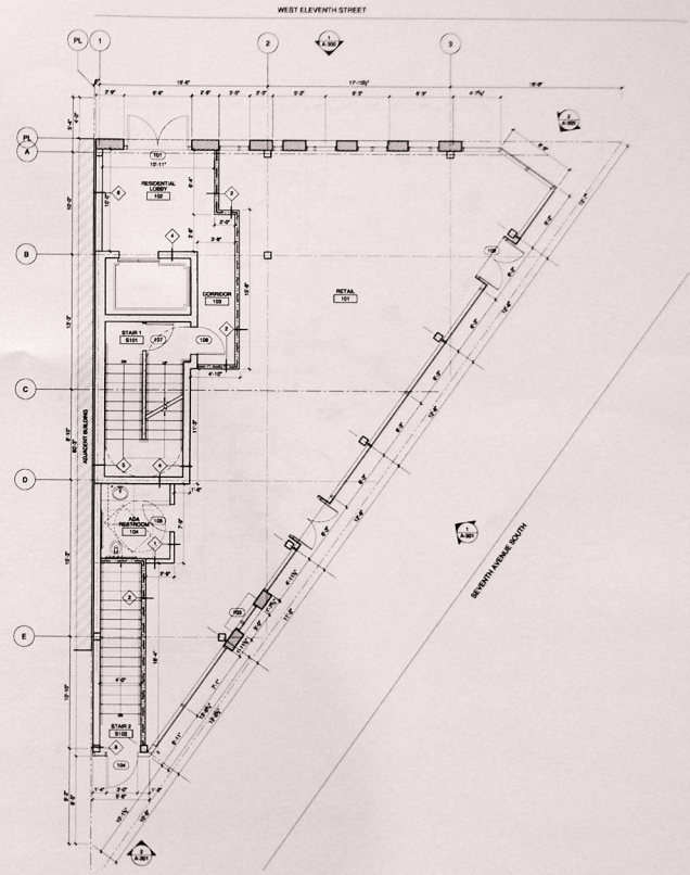
2 First Floor Plan
