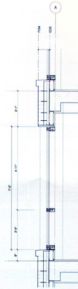
2 Section
