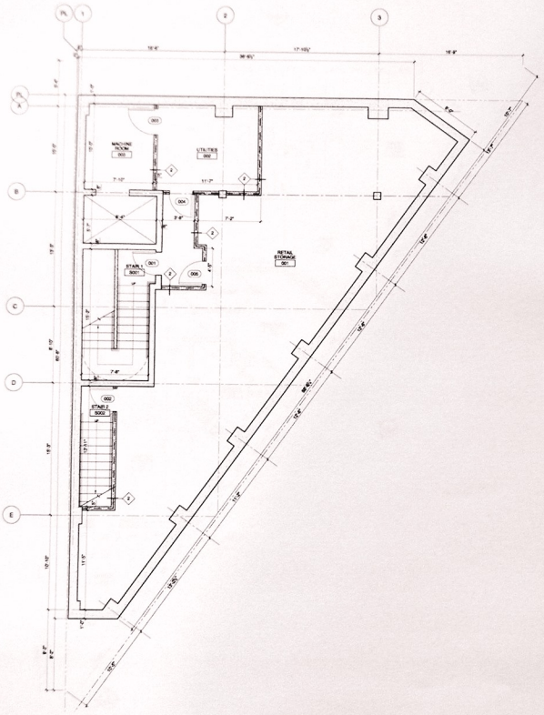
1 Cellar Plan
