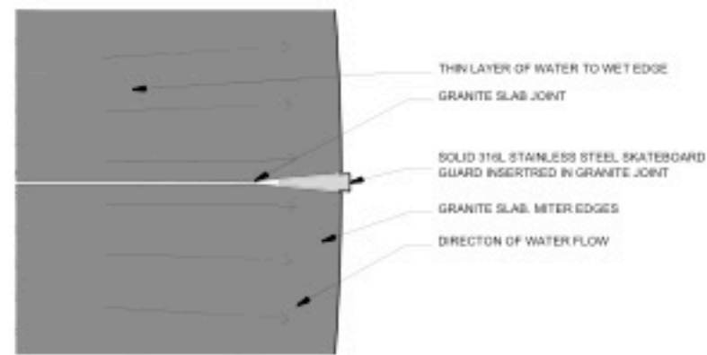
4 EDGE AND SKATEGUARD PLAN DETAIL SCALE: 1" = 1'-0"
