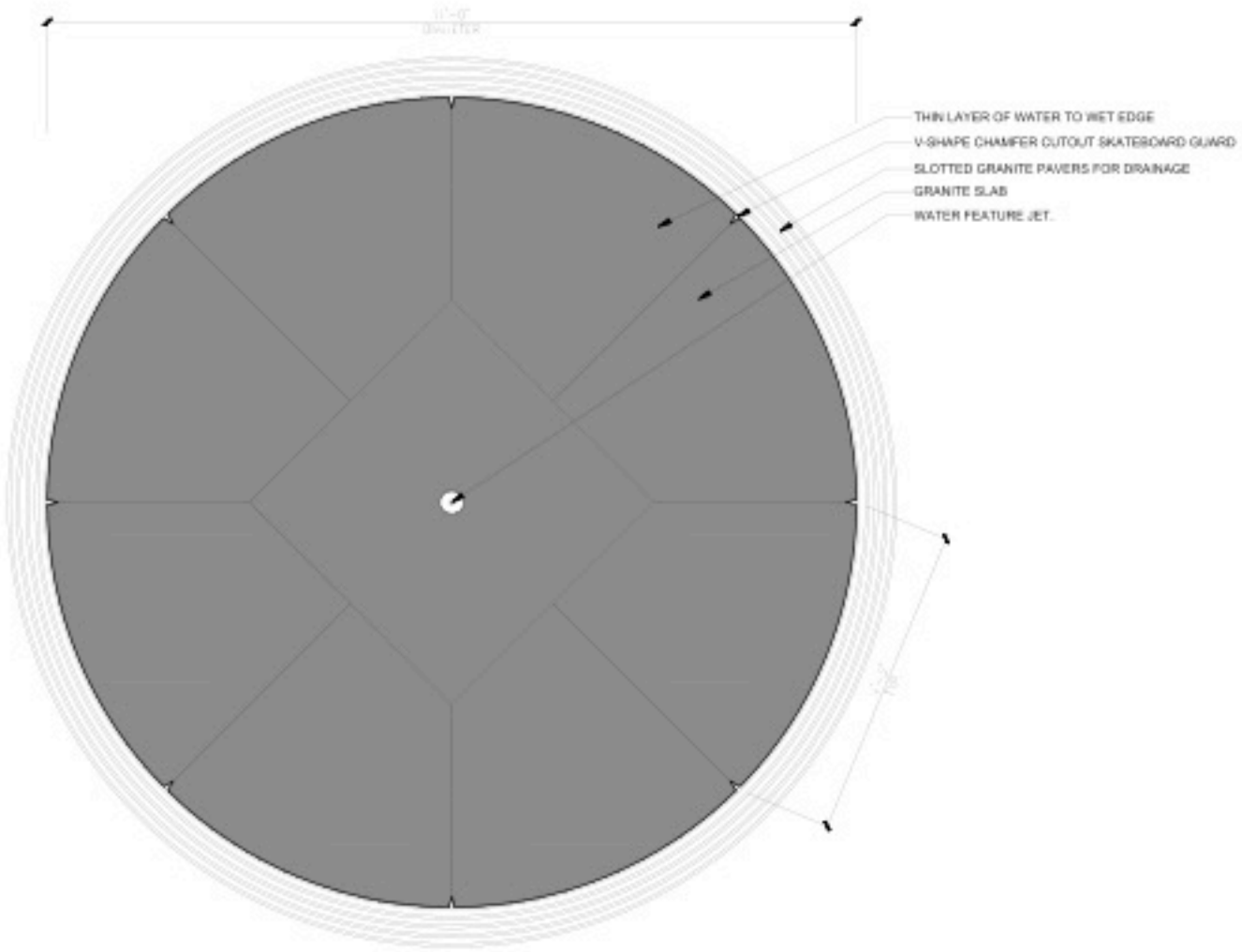
2 WATER FEATURE ENLARGED PLAN SCALE: 1" = 1'-0"
