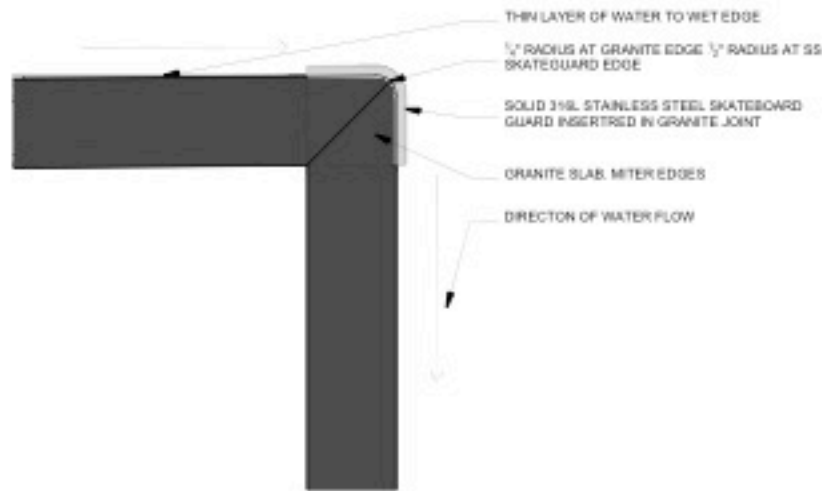
3 EDGE AND SKATEGUARD SECTION DETAIL SCALE: 1" = 1'-0"
