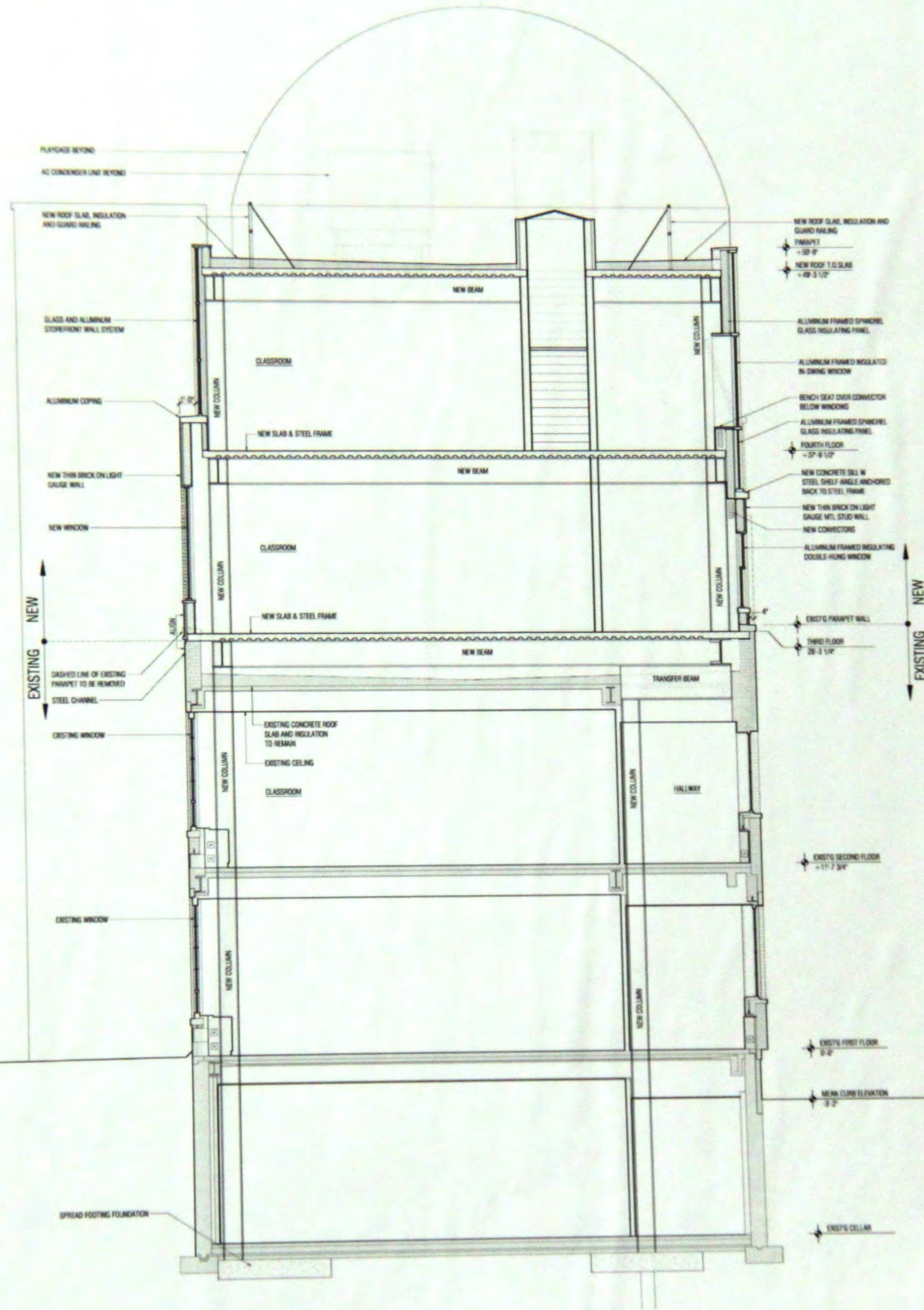
St. Luke's School at St. Luke in the Fields Typical Greenwich Street Section
