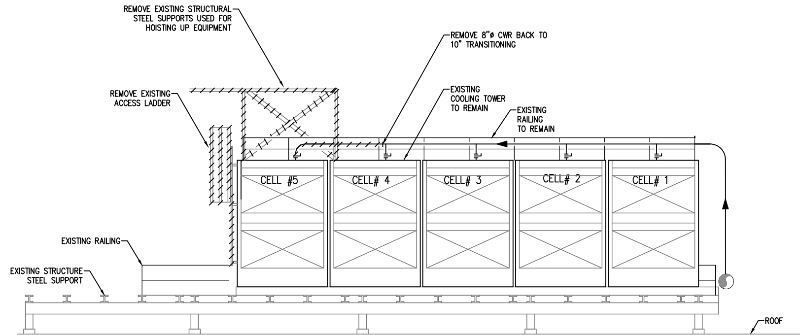
1. EXISTING COOLING TOWER SECTION
