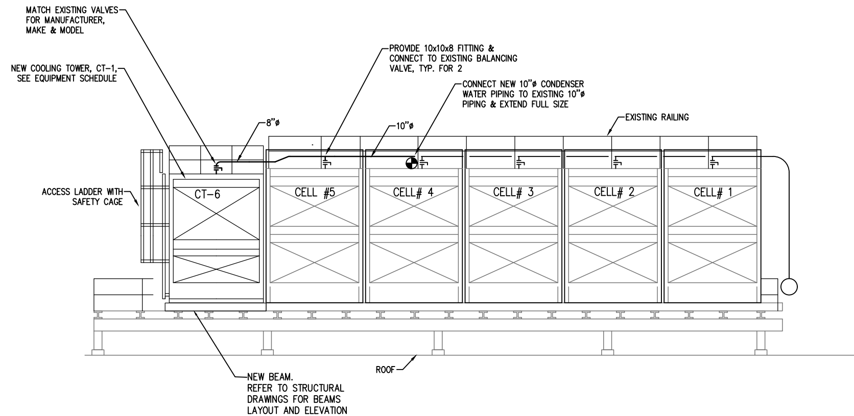
2. PROPOSED COOLING TOWER SECTION
