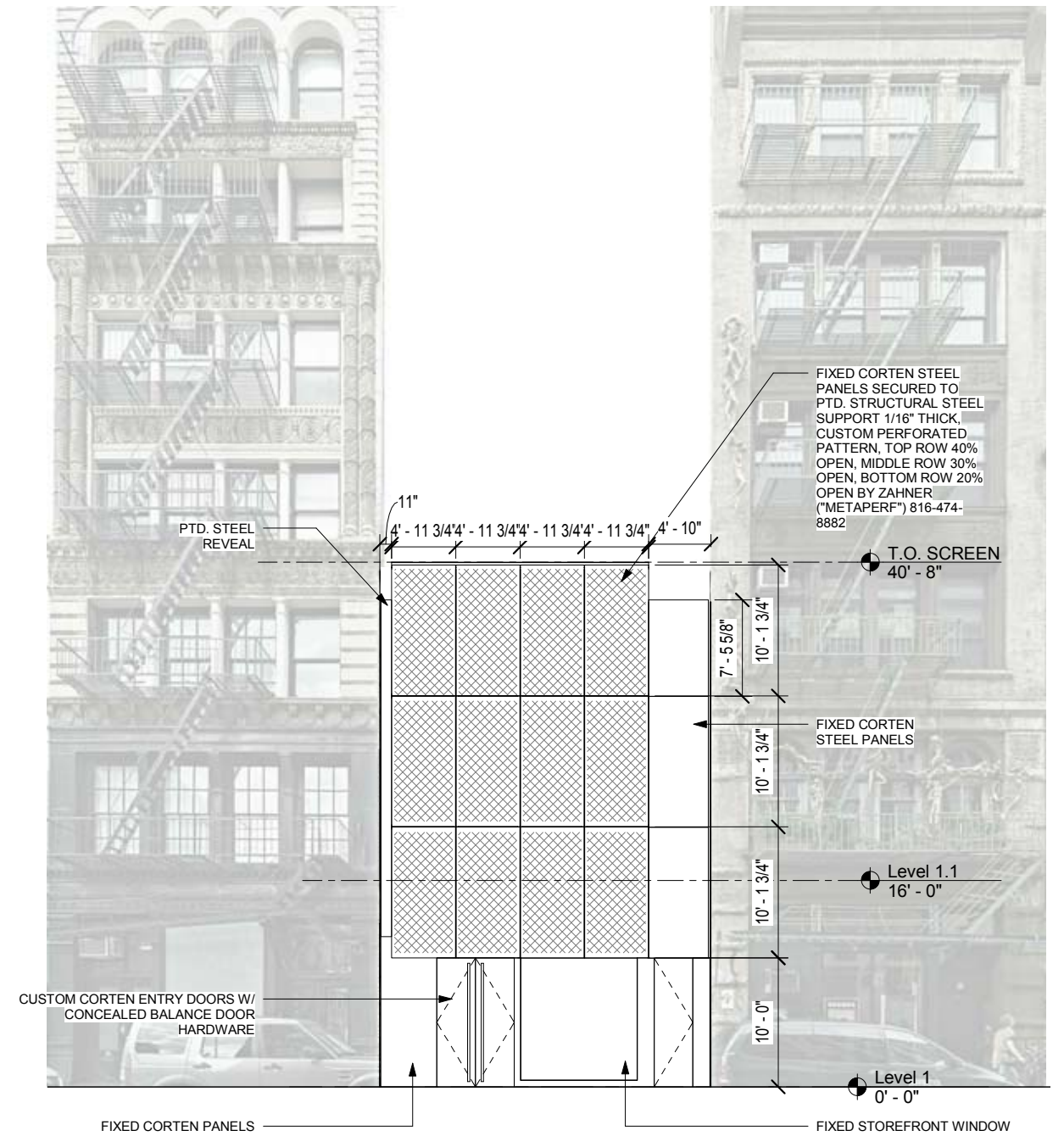
NEW PROPOSED ELEVATION - BOND ST.
