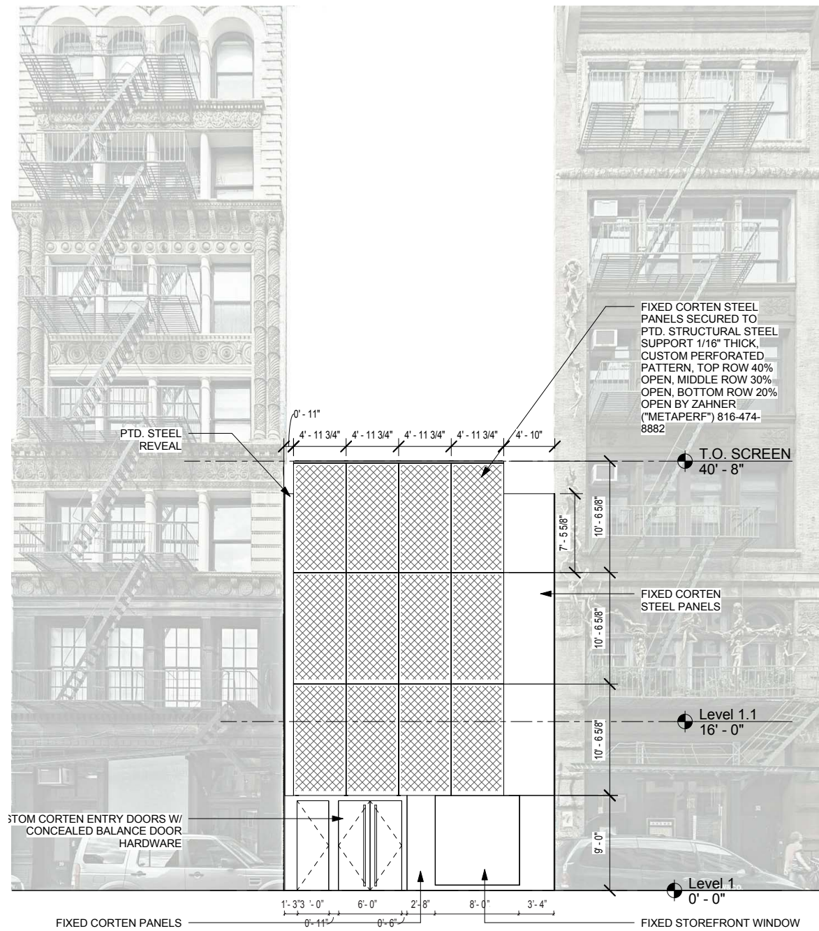
APPROVED ELEVATION - BOND ST.
