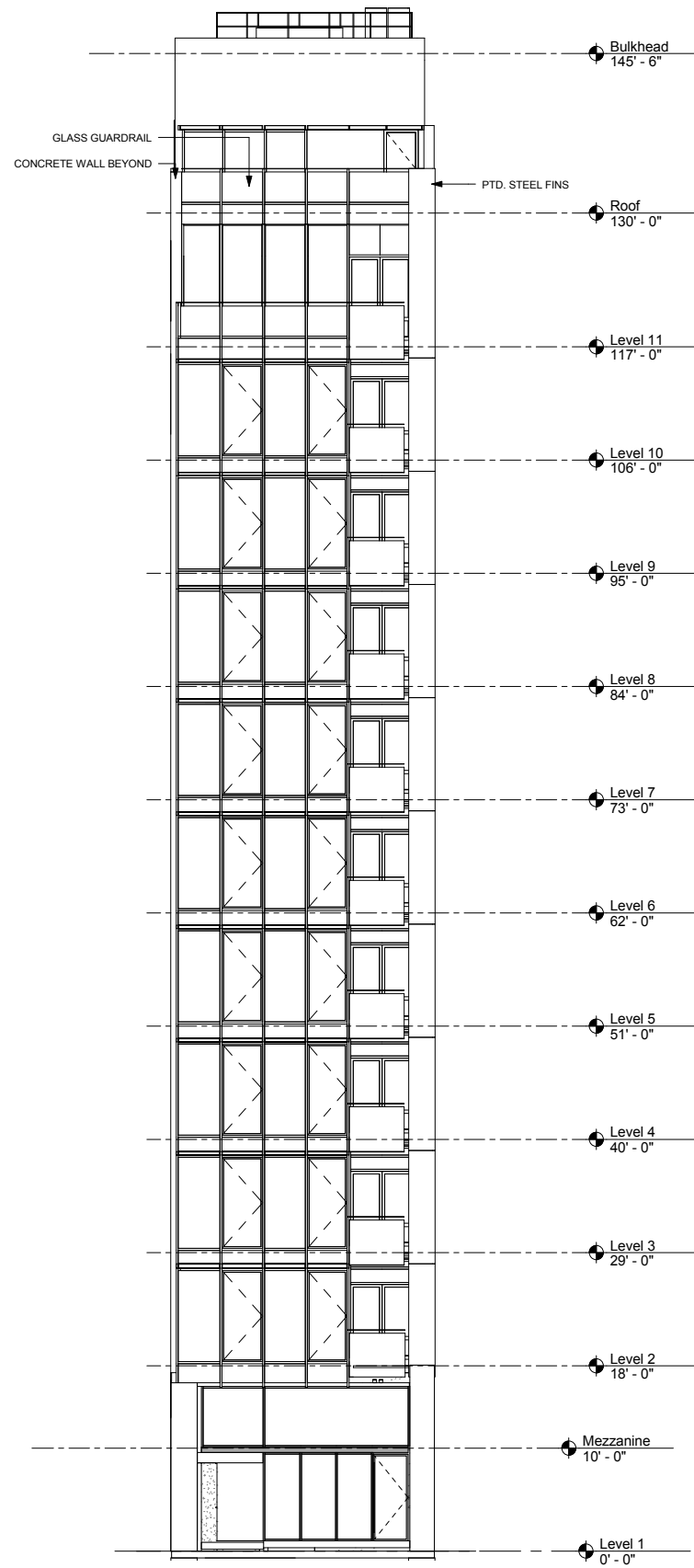
APPROVED ELEVATION
