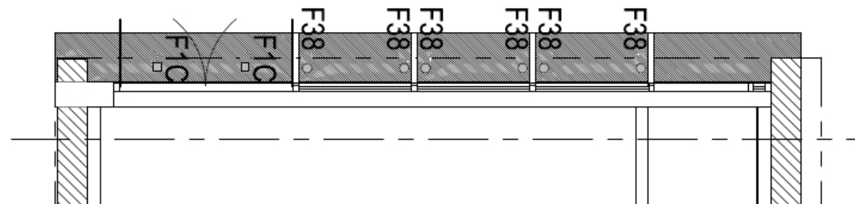
PROPOSED PLAN
