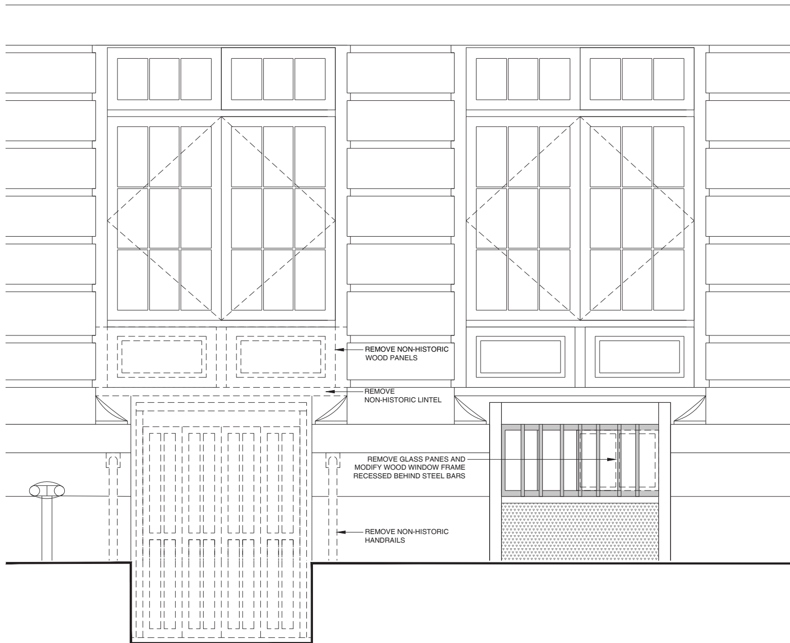
Existing - Basement Entry
