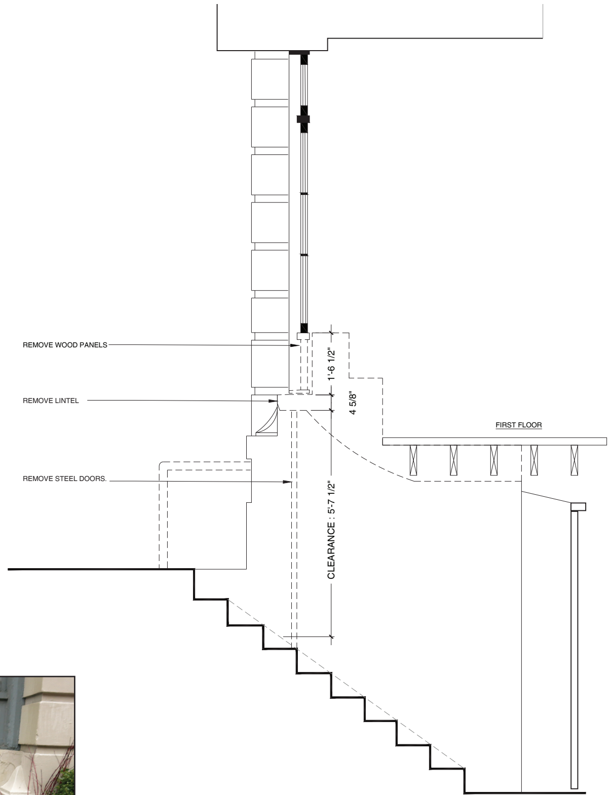
Section Through Stair
