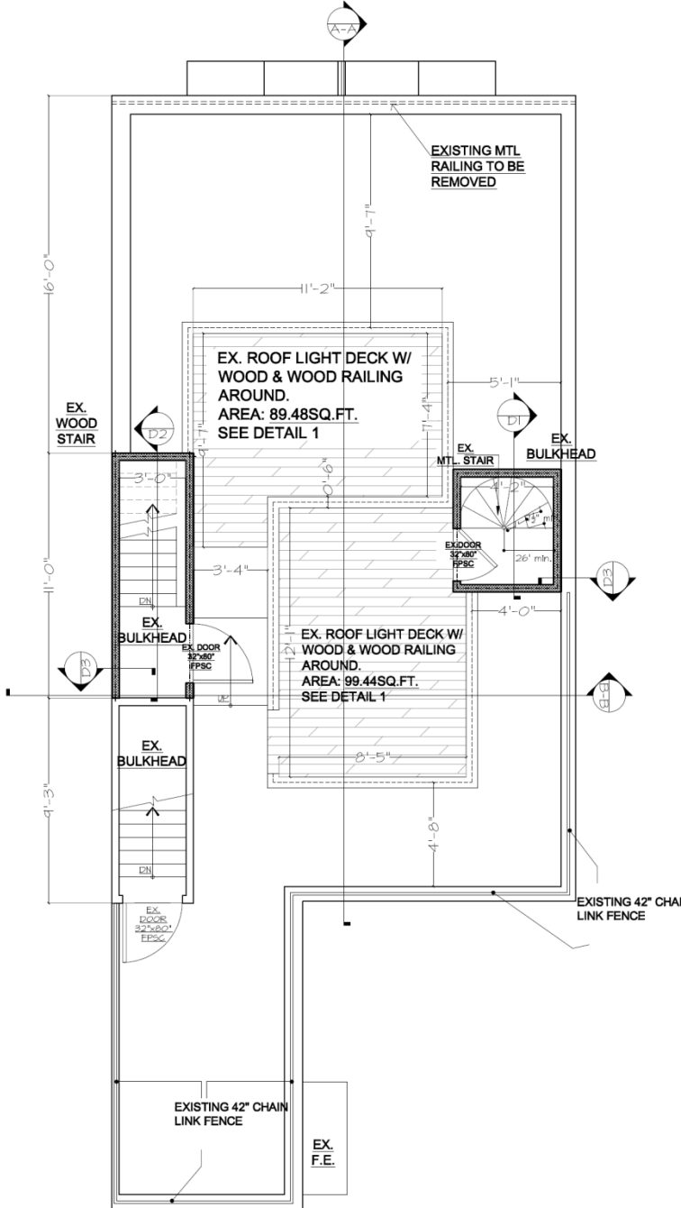
EXIST'G ROOF FLOOR PLAN SCALE: 1/4" = 1'-0"
