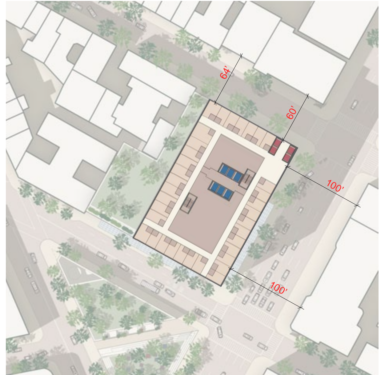
Rectangular Scheme - 8 December 2008
