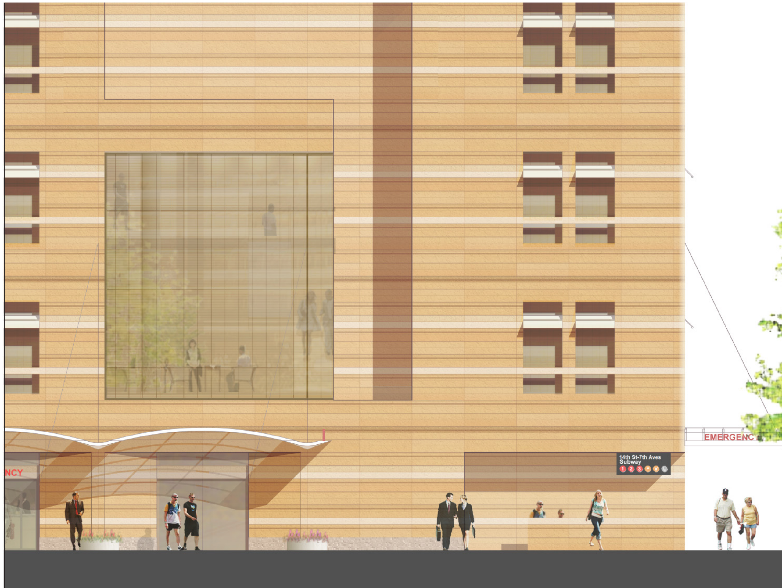
W 12th St Elevation Detail Modified Scheme - 3 June 2008
