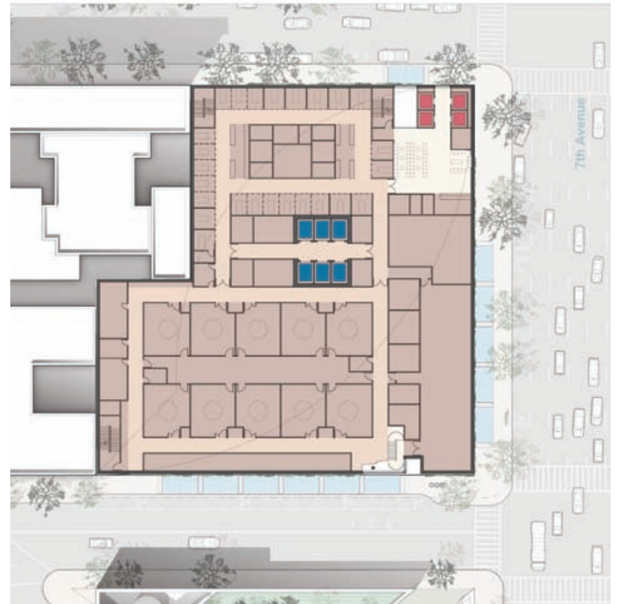
Operating Room Floor Plan - Original & Modified Scheme Similar
