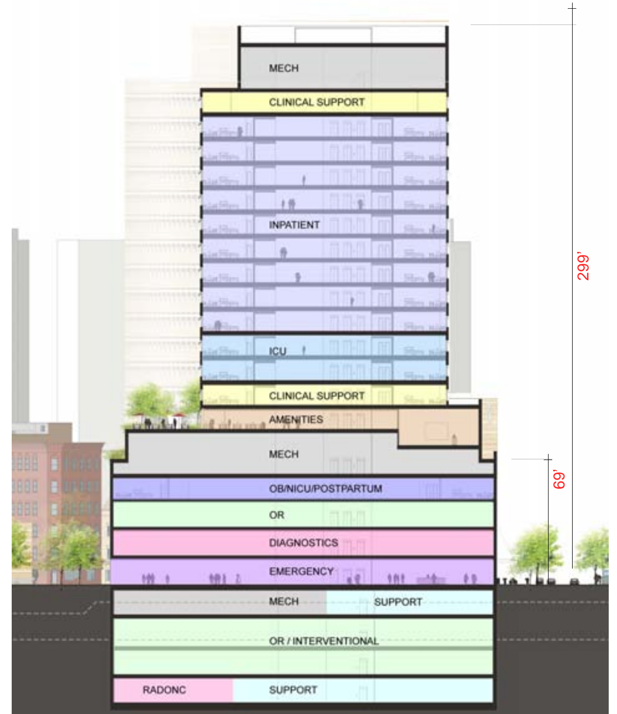
Modified Scheme - 3 June 2008
