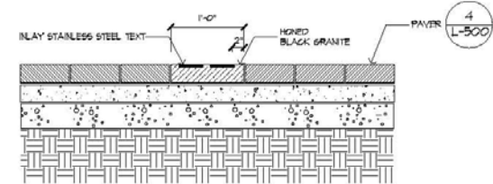
③ BLACK GRANITE PAVING DETAIL
