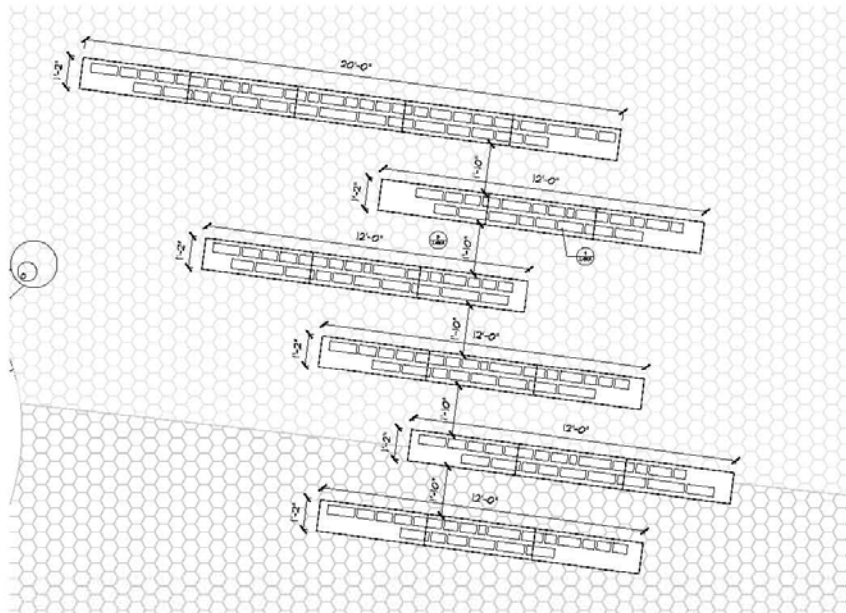
① BLACK GRANITE PAVING ENLARGEMENT
