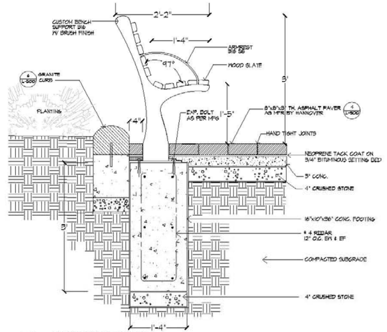
② WOOD BENCH DETAIL
