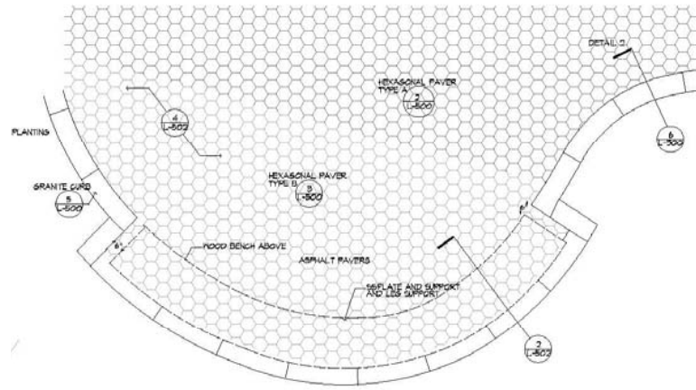
1 ASPHALT PAVERS PATTERN ENLARGEMENT
