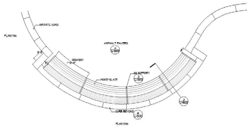
① WOOD BENCH ENLARGEMENT PLAN
