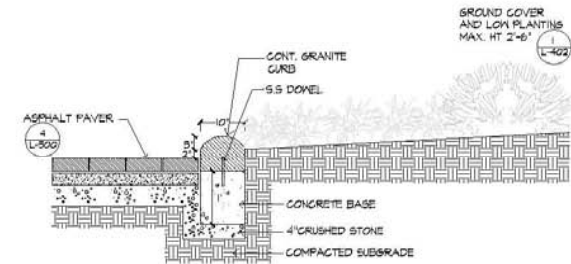
6 ASPHALT PAVERS AT CURB DETAIL
