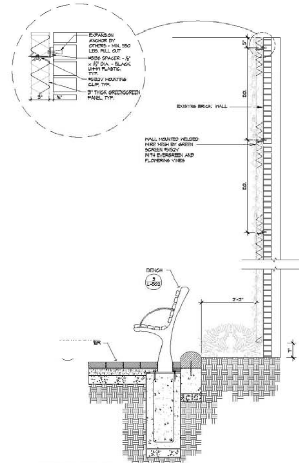
2 SECTION THRU GREENSCREEN
