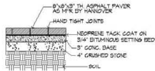
4 ASPHALT PAVERS DETAIL
